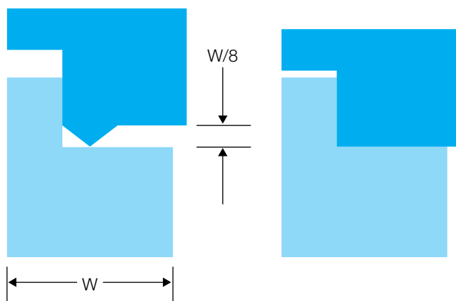
Figure 2: Step joint
