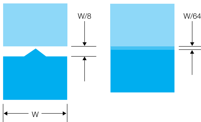
Figure 1: Butt joint
