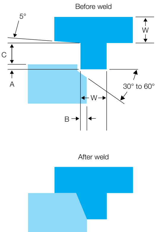
Figure 4: Shear joint
